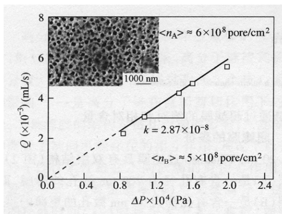
Fig. 3 Pressure difference ( \Delta P ) dependence of macroscopic flow rate ( Q ) of toluene and the; Inset shows SEM image of surface of layer A in Fig. 2
