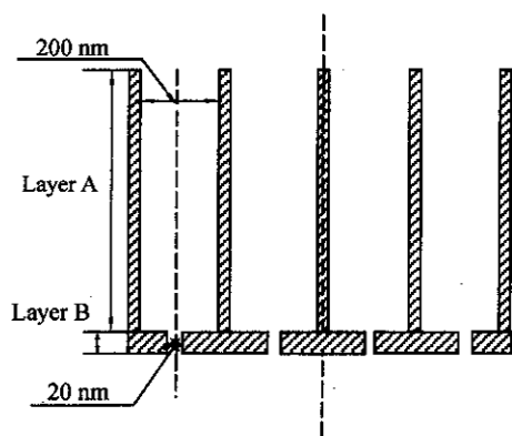
Fig. 2 Schematic of the membrane filter used (not in a proportional scale)
