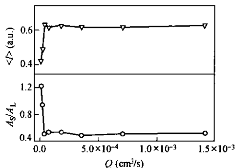
Fig. 6 Macroscopic flow rate ( Q ) dependence of time average intensity ( \langle I \rangle ) and area ratio of two peaks ( A_S/A_L ) in hydrodynamic radius distribution
