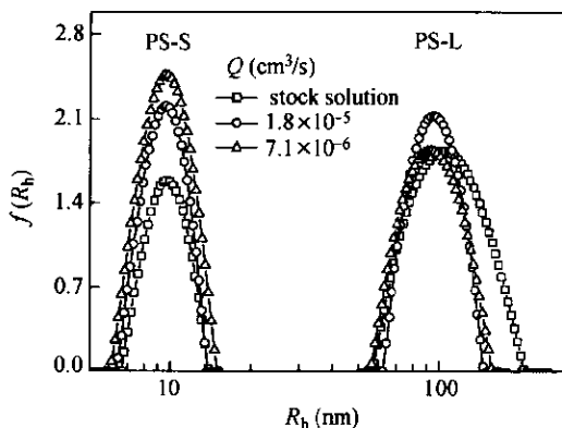
Fig. 8 Flow rate ( Q ) dependence of hydrodynamic radius distributions, where Q is lower than the macroscopic threshold flow rate ( Q = 1.8 \times 10^{-5} \text{ cm}^3/\text{s} )
