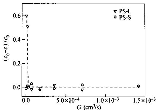
Fig. 7 Macroscopic flow rate ( Q ) dependence of retention concentrations of PS-S and PS-L
