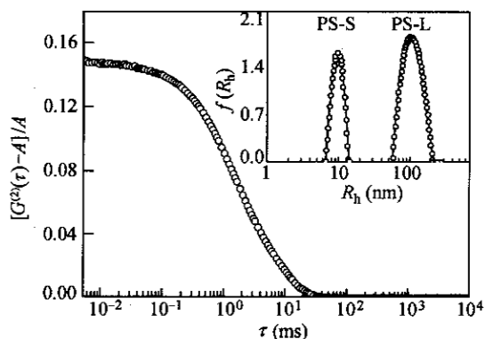
Fig. 4 Intensity auto-correlation function of a solution mixture of shorter polystyrene chains (PS-S) and longer polystyrene chains (PS-L); Inset shows a corresponding distribution of hydrodynamic radius ( R_h ) calculated from Laplace inversion of [G^{(2)}(\tau) - A]/A
