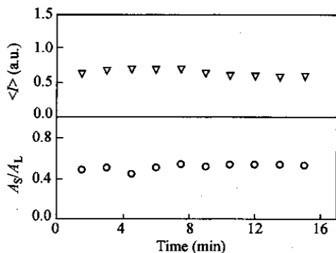
Fig. 5 Time dependence of time average intensity ( \langle I \rangle ) and area ratio of two peaks ( A_s/A_L ) in hydrodynamic radius distribution during ultra-filtration of a solution mixture of PS-S and PS-L
